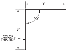
AAFN3310, GAFN3310
